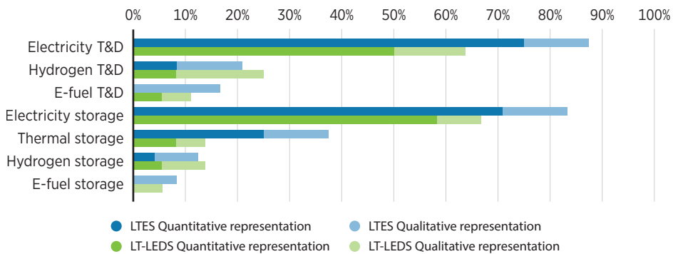
Figure 8 Representation of power, hydrogen and e-fuel transmission & distribution and storage in LTES and scenario-based LT-LEDS scenarios
